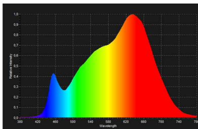
White 3000° Curve
