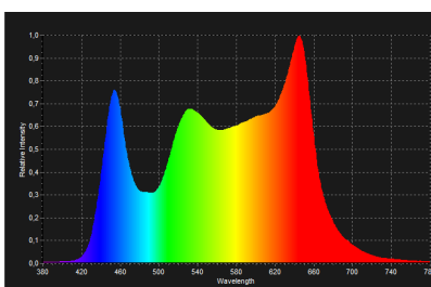
Curva White 4000°
